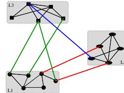
Fig. 2. A multicolored multi-layer network with 3 layers (L1, L2, L3).
